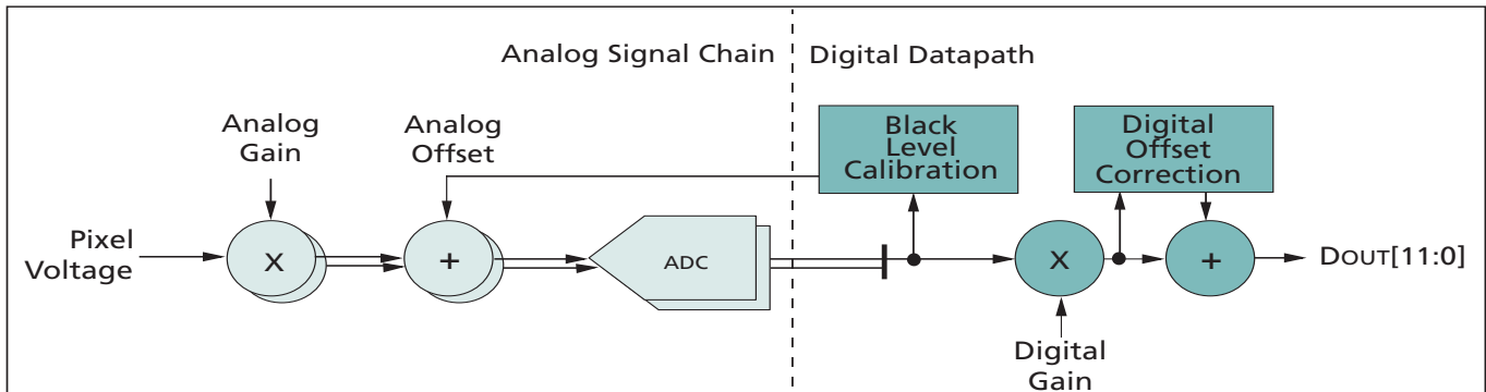
Figure 25: Signal Path
