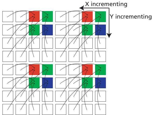
Figure 20: Pixel Readout (Column Bin 2X, Row Bin 2X)
