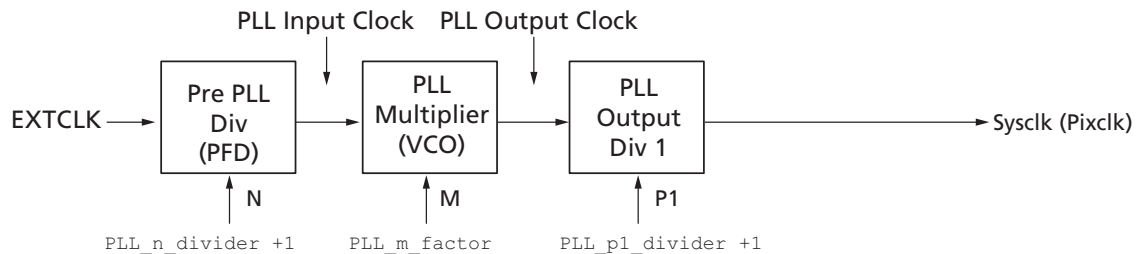
Figure 13: PLL Generated Master Clock
