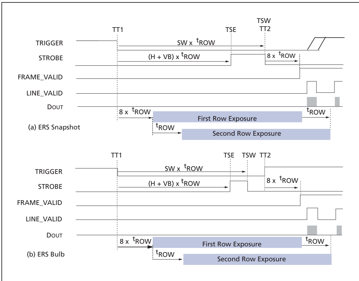
Figure 23: ERS Snapshot Timing
