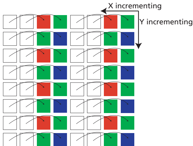
Figure 19: Pixel Readout (Column Bin 2X)
