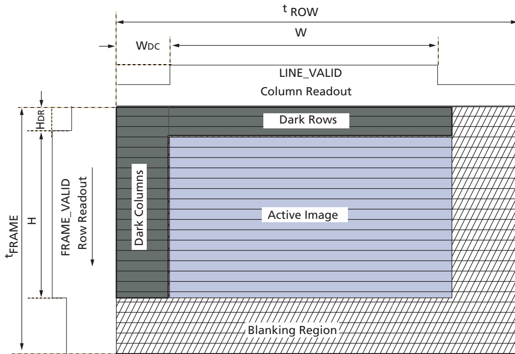
Figure 10: Frame Timing
